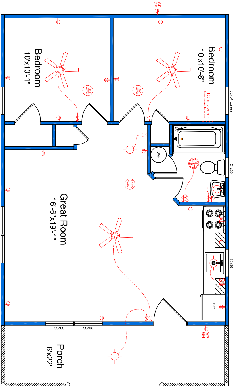
Plan 22CC501-B 22'x36' with 6' porch included
